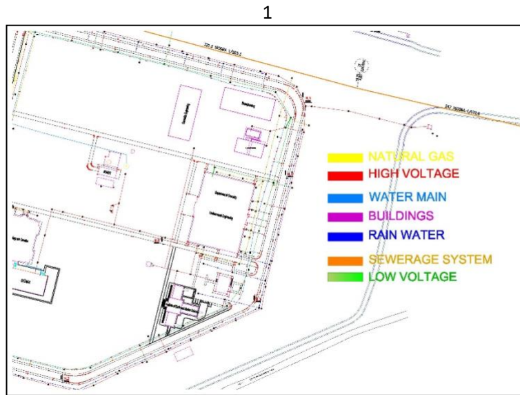
1-sewage system pipes (orange color lines) from the GTU campus to the Gebze wastewater treatment plant which is 1 km away from the campus
